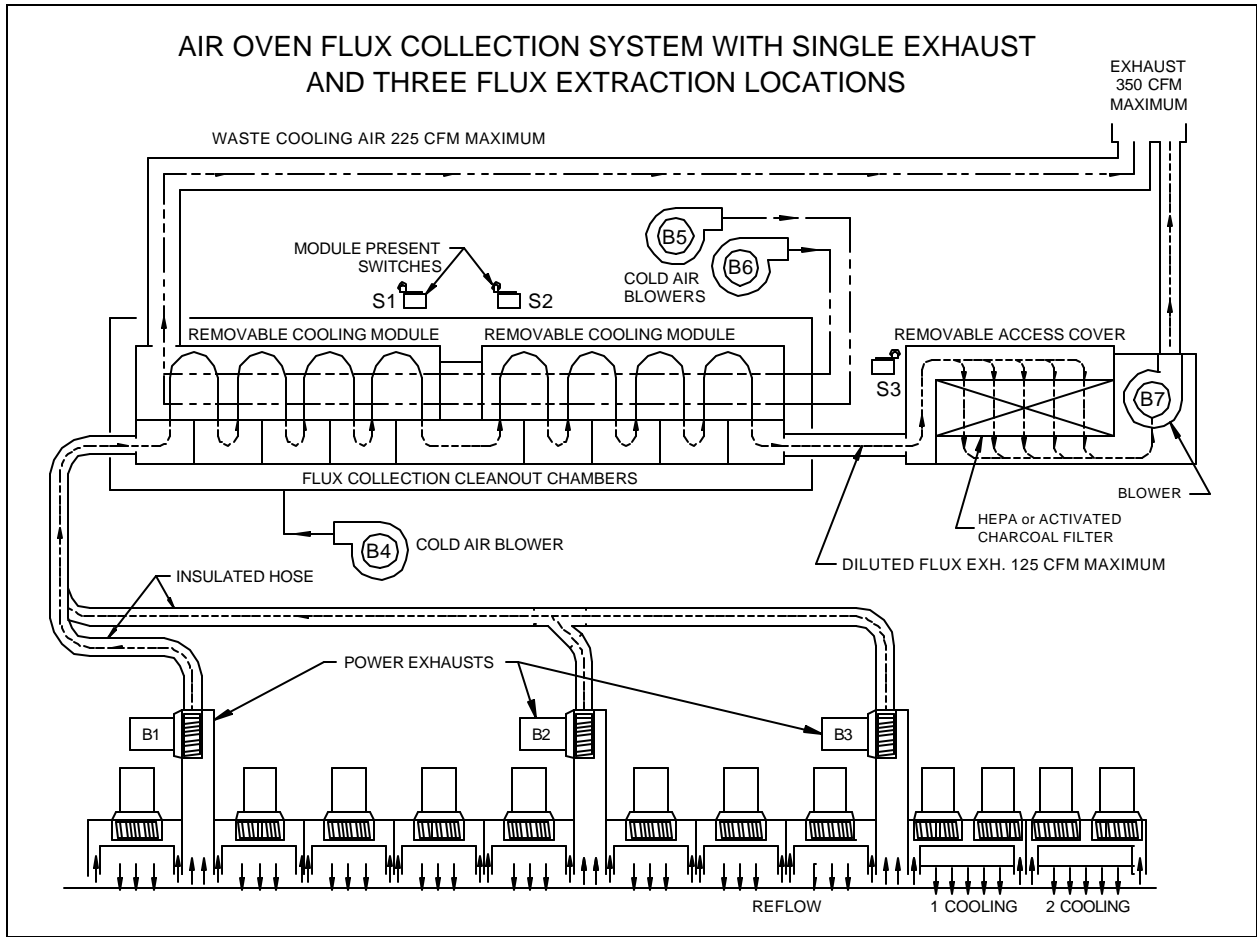
Figure 8: Filtered Air Flux Collection System with Three Extraction Locations.
